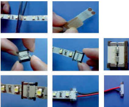
Joining connector
